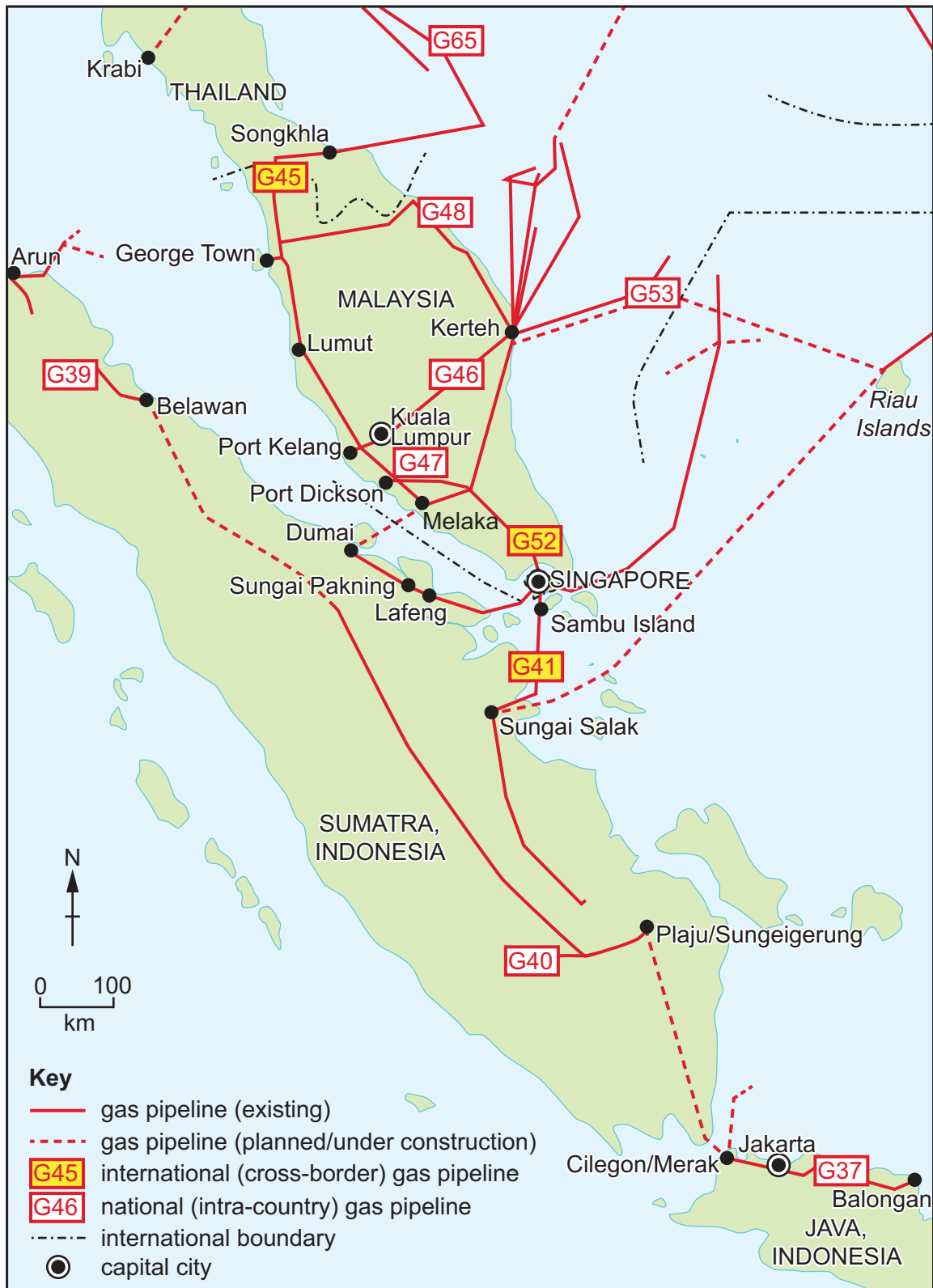
Natural gas pipelines in part of Southeast Asia, 2017
